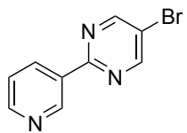
6 ^1\text{H} NMR 400 MHz, \text{CDCl}_3
